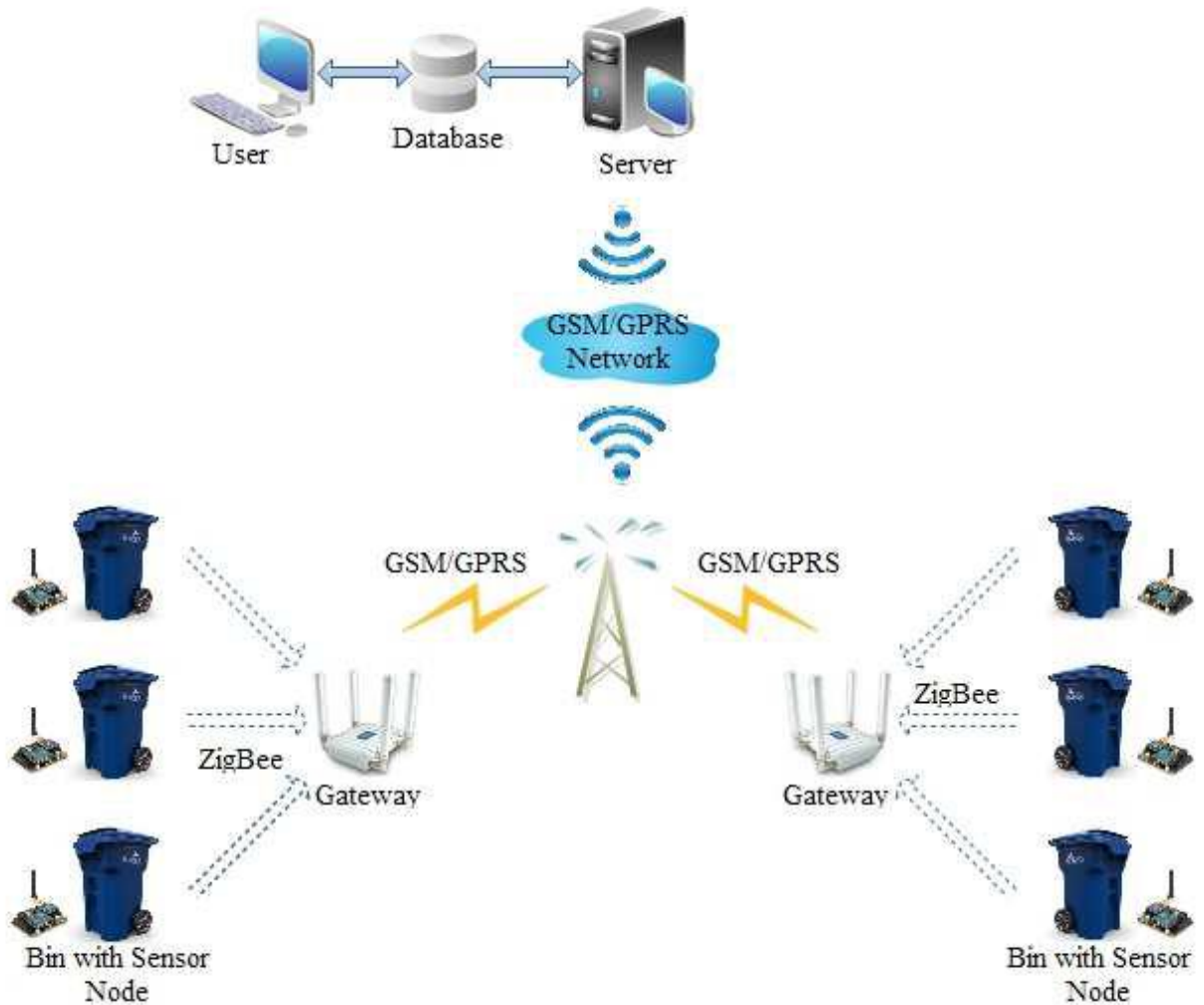
Figure 2.1: Automated Solid Waste Bin Monitoring System Framework
