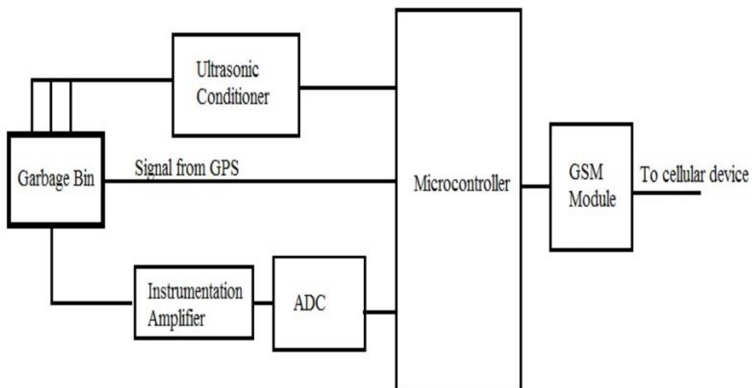
Figure 2.3: Block diagram for Smart Garbage Bin
