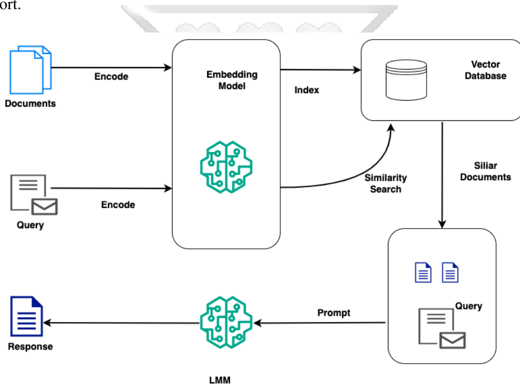
Figure 2.9: RAG Workflow implemented using Azure AI Studio
