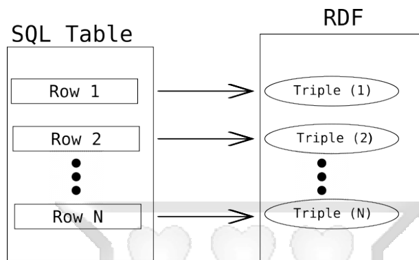
FIGURE 3.2: Parsing SQL to RDF. The parser operates on each row in a SQL table to produce a valid triple store.
