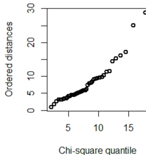
Chiplot for Cereals Data
