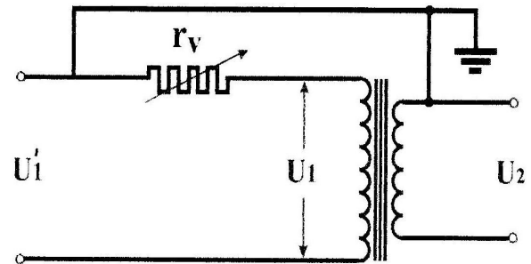
Fig.8. Circuit for the Dispersion Measurement
