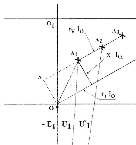
Fig.9. Determination of x_1 and the Compensation
