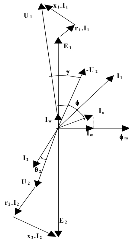
Fig. 5. Phasor Diagram of the Transformer
