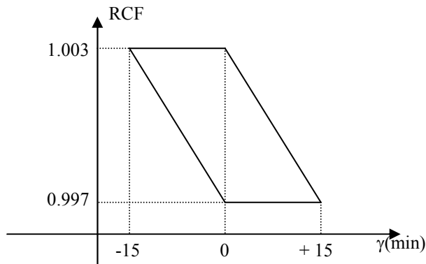
Fig. 1. Limits of Accuracy for a 0.3 Class Voltage Transformer for Metering Service
