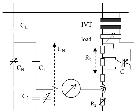
Fig. 2. Capacitive Divider Circuit
