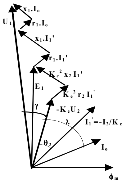
Fig. 6. Phasor Diagram Referred to the Primary Side of the Transformer
