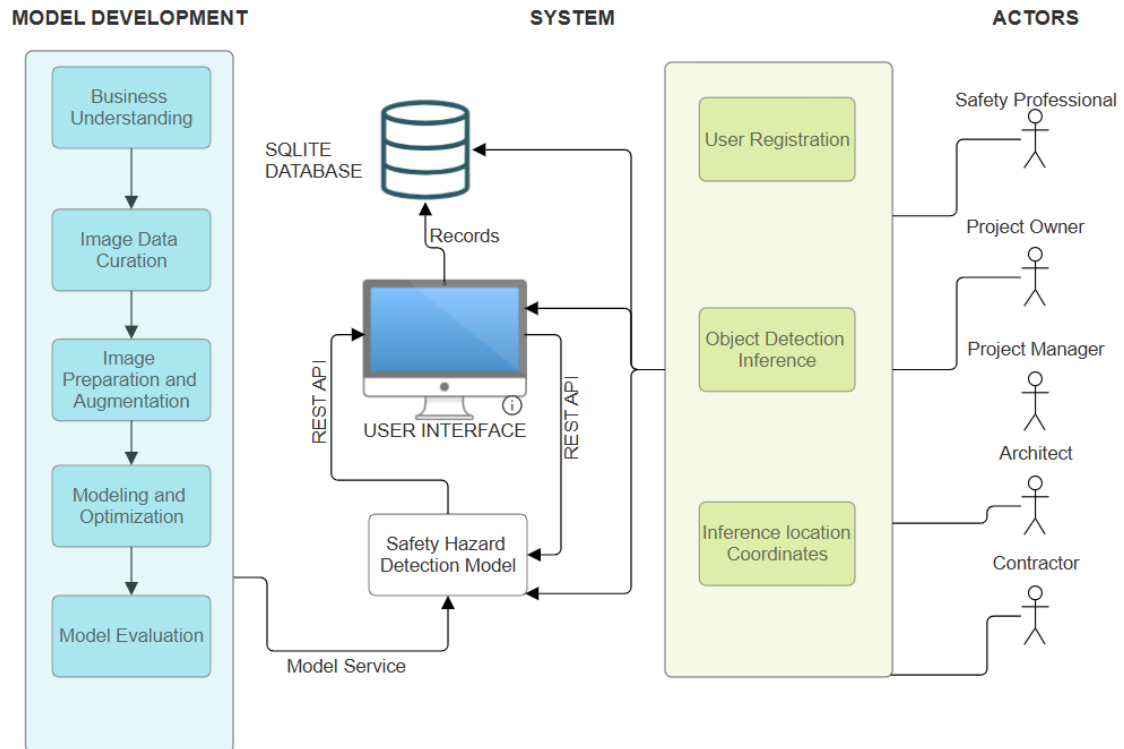
Figure 4.1: UML diagram
