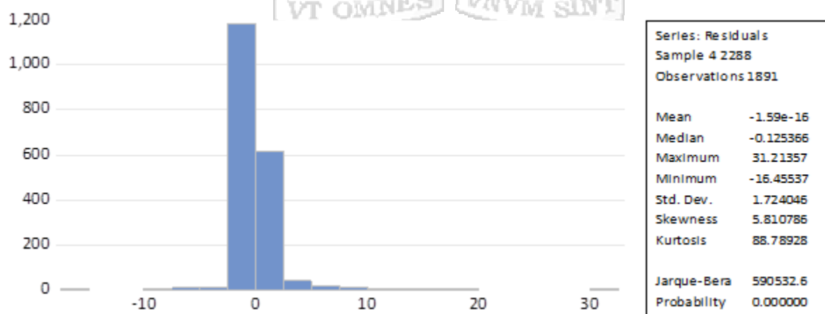
Figure 4.1 Normality Test
