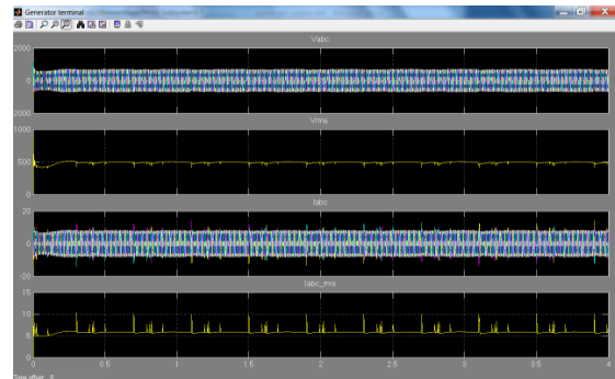
Figure 5: Induction generator output
