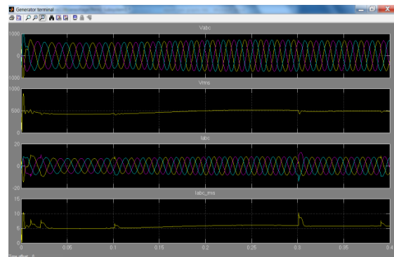
Figure 6: IG terminal voltage and current
