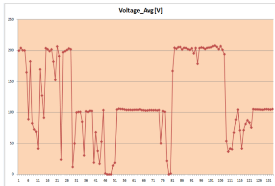
Figure 12: Voltage characteristics
