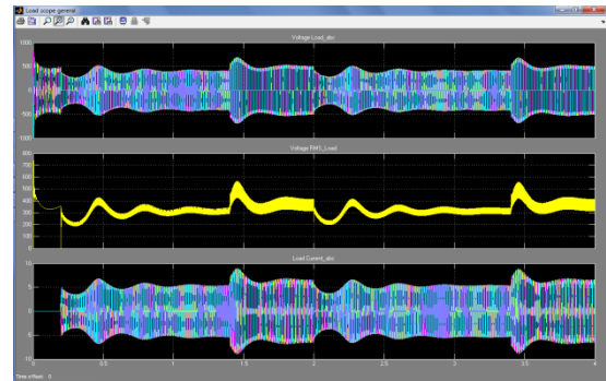
Figure 10: Load terminal volatge and current wave forms
