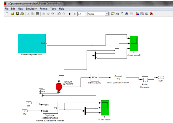
Figure 42: Error calculation and PID controller
