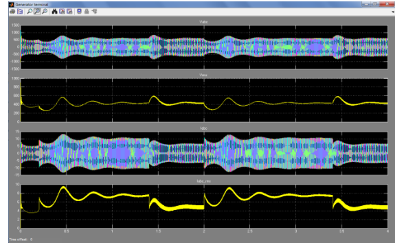
Figure 9:IG voltage and current waveforms
