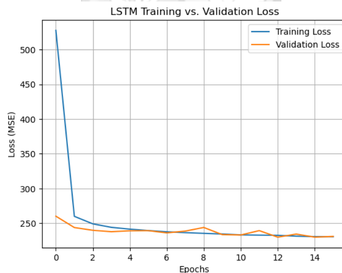
Figure 4.5: Training vs. Validation Loss for the LSTM Model
