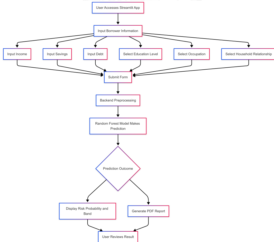
Figure 4.3: User Interface Data Flow in Credit Scoring Application
