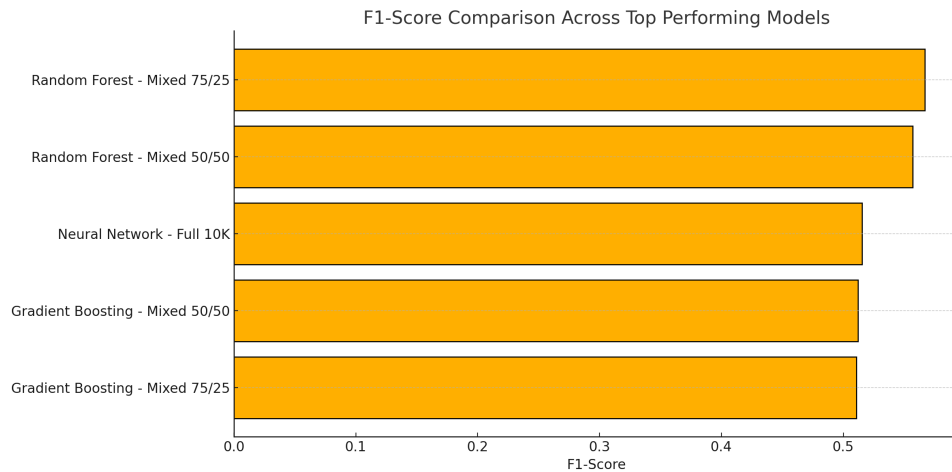
Figure 6.10: F1-Score Comparison Across Top Performing Models
