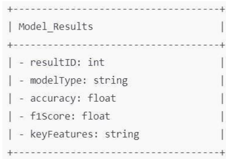
Figure 4.6: Model_Results Class
